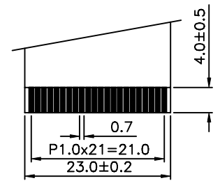
FFC CONTACT SIDE DETAILS
