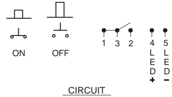
CIRCUIT
