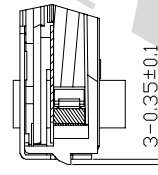
SECTION Dd-Dd SCALE 4:1
