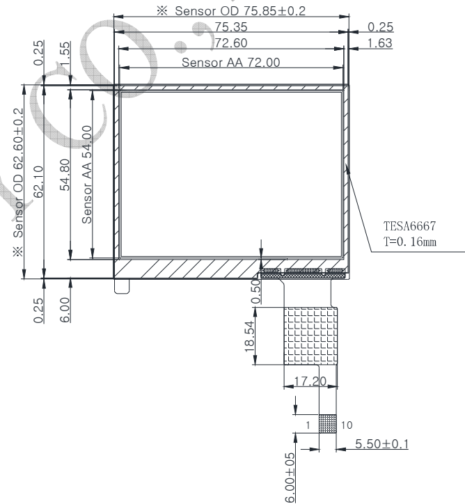
BACK VIEW
